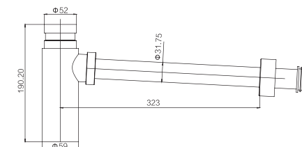
GY02066 Bottle trap 1 1/4" & 1 1/2" CP / ORB /BLACK/BN .ETC Brass
