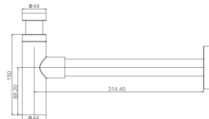
GY02054 Bottle trap 1 1/4" & 1 1/2" CP / ORB /BLACK/BN .ETC Brass
