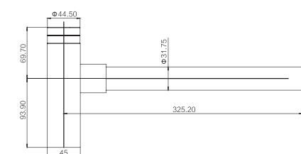
GY02041 Bottle trap 1 1/4" & 1 1/2" CP / ORB /BLACK/BN .ETC Brass
