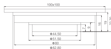
GY01913 Floor drain CP / PB /ORB / BN . ETC Brass
