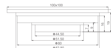
GY01914 Floor drain CP / PB /ORB / BN . ETC Brass
