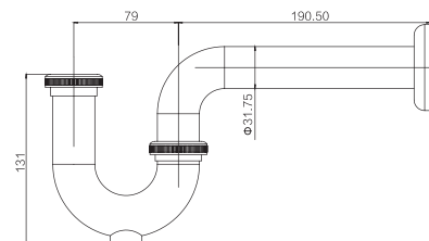
GY05040 P Trap 1 1/4" & 1 1/2" CP / ORB /BLACK/BN .ETC Brass & Stainless steel
