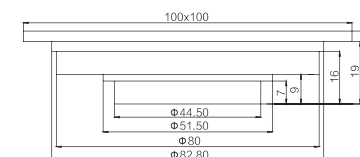
GY01908 Floor drain CP / PB /ORB / BN . ETC Brass
