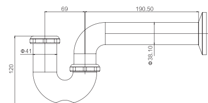
GY05008 P Trap 1 1/4" & 1 1/2" CP / ORB /BLACK/BN .ETC Brass & Stainless steel
