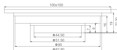
GY01911 Floor drain CP / PB /ORB / BN . ETC Brass
