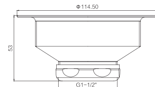
GY04003 Kitchen drain 1 1/2" CP/ORB/ BLACK/BN/SN.ETC Brass & Stainless Steel
