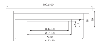
GY01910 Floor drain CP / PB /ORB / BN . ETC Brass
