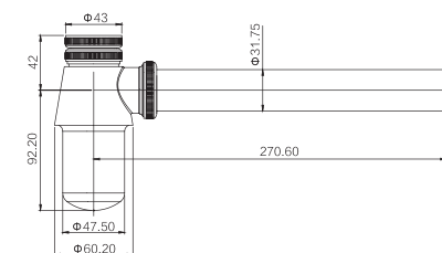
GY02033 Bottle trap 1 1/4" & 1 1/2" CP / ORB /BLACK/BN .ETC Brass
