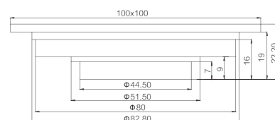
GY01912 Floor drain CP / PB /ORB / BN . ETC Brass
