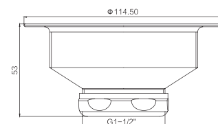
GY04001 Kitchen drain 1 1/2" CP/ORB/ BLACK/BN/SN.ETC Brass & Stainless Steel
