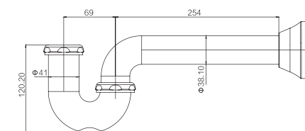
GY05001 P Trap 1 1/4" & 1 1/2" CP / ORB /BLACK/BN .ETC Brass & Stainless steel
