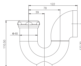
GY05026 P Trap 1 1/4" & 1 1/2" Nature brass / CP / ORB /BLACK/BN .ETC Brass & Stainless steel
