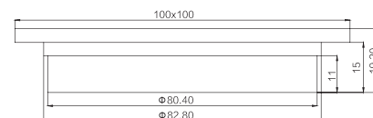
GY01904 Floor drain CP / PB /ORB / BN ETC Brass
