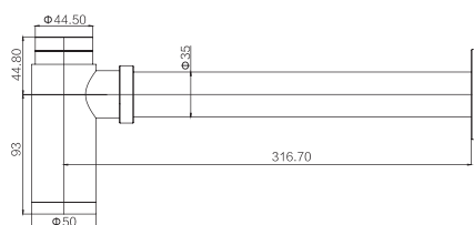
GY02055 Bottle trap 1 1/4" & 1 1/2" CP / ORB /BLACK/BN .ETC Brass
