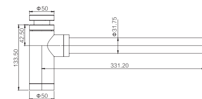
GY02034 Bottle trap 1 1/4" & 1 1/2" CP / ORB /BLACK/BN .ETC Brass
