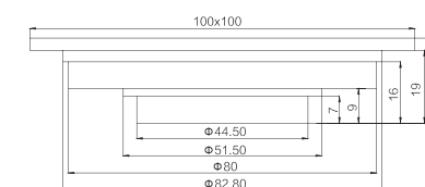
GY01909 Floor drain CP / PB /ORB / BN . ETC Brass
