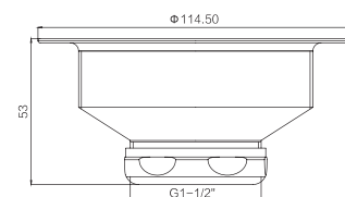
GY04004 Kitchen drain 1 1/2" CP/ORB/ BLACK/BN/SN.ETC Brass & Stainless Steel
