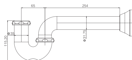
GY05002 P Trap 1 1/4" & 1 1/2" CP / ORB /BLACK/BN .ETC Brass & Stainless steel
